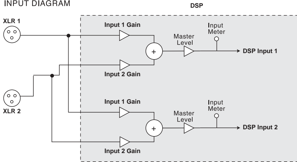
INPUT DIAGRAM
